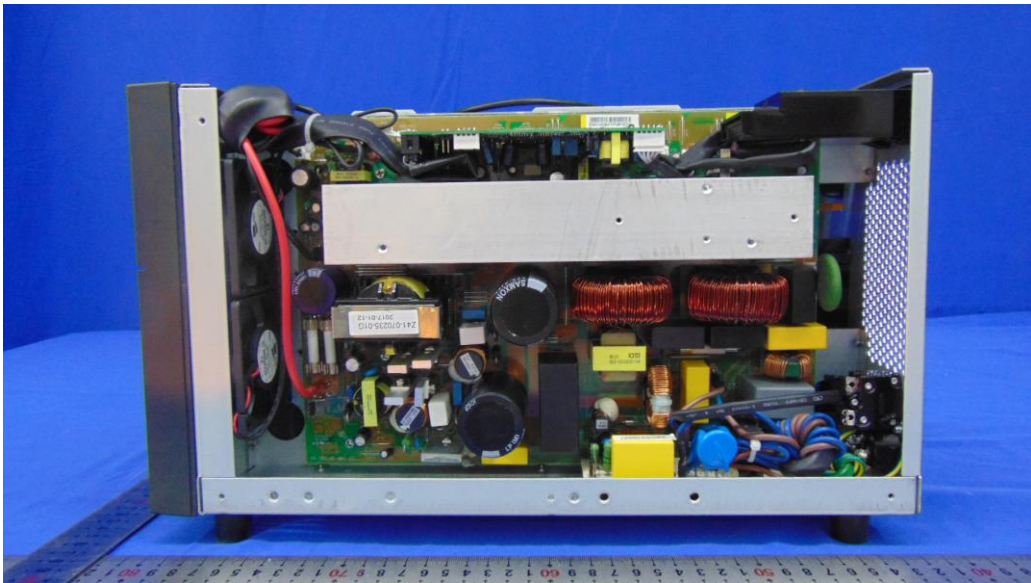
Figure 11 General Internal of the E.U.T.
