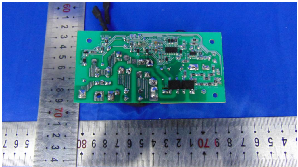
Figure 20 General Appearance of the PCB
