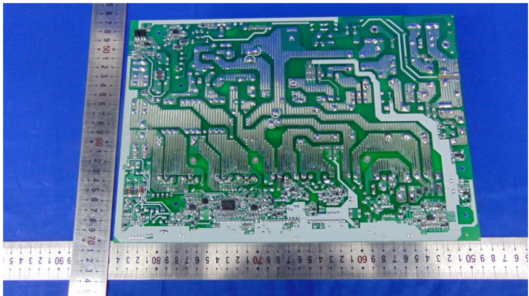
Figure 16 General Appearance of the PCB
