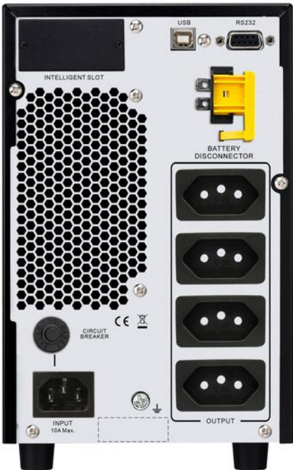
Figure 7 General Appearance of the E.U.T.
